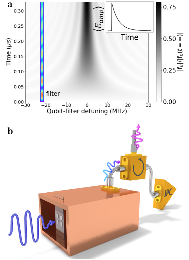
Figure 1: The idea of the visualization of the photon emission with frequency and time resolved spectroscopy. a , Visualization of formula 2: single photon spectrum, as a function of time, i.e. set of |f_{\mathbf{k}}(t)| in Wigner-Weisskopf theory, which is proportional to the electric field amplitude E_{\mathbf{k}} , corresponding to the wave vector \mathbf{k} . Along the x-axis we plot the qubit detuning from the mode \mathbf{k} : \omega_{\mathbf{k}} - \omega_q . The plot is normalized by |f_0(t = \infty)| , corresponding to zero detuning. For the plot we used \gamma/2\pi = 1.5\text{MHz} and assumed g_{\mathbf{k}} to be constant within the vicinity of the qubit frequency. The colored area is strongly amplified by the narrow-band quantum limited amplifier (JPC), playing the role of the filter. The JPC allows to visualize the entire picture line by line by sweeping the qubit detuning relative to the JPC resonance. The inset depicts the electric field amplitude \langle E_{\text{amp}} \rangle (integrated over all frequencies) of the same signal. b , Experimental setup. Two transmon qubits are coupled to the fundamental mode of a copper waveguide with rectangular cross section. The coherent drive is applied to the qubits through the waveguide (blue wavy arrow). After the abrupt stop of the drive the system emits a relatively broadband signal (see the inset on the subplot a ). The particular frequency component which is being amplified by the JPC is shown by the pink wavy arrow.
