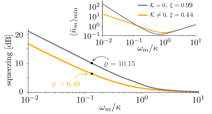
FIG. 11. Squeezing for optimal cooling as a function of the resolved-sideband parameter for the nonlinear (orange line) and linear (gray line) case, using a purity of squeezing of \xi = 0.44 and 0.99 , respectively. The two black dots denote the respective squeezing strengths at \omega_m/\kappa = 0.13 discussed in the text. The inset shows the corresponding minimum phonon number as a function of the resolved parameter. Here mechanical occupation below one is obtained at \omega_m/\kappa = 0.13 , where both lines intersect. For the plots we used g_0/2\pi = 15 kHz and the remaining parameters are as in Table I.
