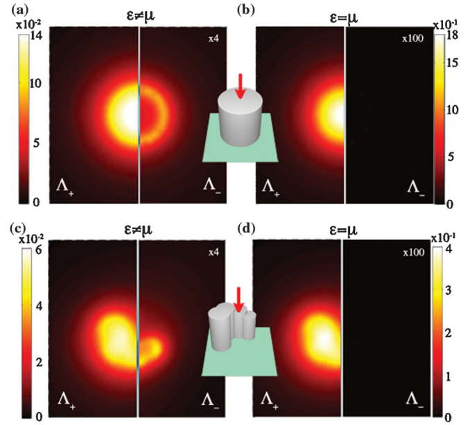
FIG. 1 (color). Impact of the different symmetries on the field scattered by two dielectric structures. The upper row shows the scattered intensity for a symmetric cylinder and the lower row for a pan-flute-like shape without any rotational, translational, or spatial inversion symmetry. The length and diameter of the cylinder are 200 nm. The pan flute is made of cylinders of different lengths and diameters; the longest one is 200 nm long and the total pan flute's width is around 200 nm. In panels (a) and (c), the structures have \epsilon = 2.25 , \mu = 1 , while in panels (b) and (d) we enforced duality symmetry by setting \epsilon = \mu = \epsilon_{\text{glass}} = 2.25 . The incident field is a plane wave of well-defined helicity equal to 1, a momentum vector pointing to the positive z axis, and a wavelength of 633 nm. Its electric field is (\hat{x} + i\hat{y})/\sqrt{2} \exp(kz - \omega t) . The left-half side of each subfigure corresponds to the scattered field with helicity equal to the incident plane wave \Lambda_+ ; the right half is for the opposite helicity \Lambda_- . The intensities of the two helicities ( \pm ) are computed as |\mathbf{E} \pm i\mathbf{H}|^2 . In [13] (see Sec. 2.1), it is shown that \mathbf{E} \pm i\mathbf{H} (with our choice of units) separates the two helicity components. The calculation plane is perpendicular to the z axis and 20 nm away from the surface of the scatterers opposite to the one where the incident field comes from. The calculation area is 700 \times 700 nm. For color scaling purposes, the right-half side is multiplied by the factor in the upper right corner. The (lack of) cylindrical symmetry of the structures results in (non-)cylindrically symmetric field patterns, which is consistent with the geometry of each case. On the other hand, both scatterers behave identically with respect to the conservation of helicity, which is seen to depend exclusively on the electromagnetic properties of the material. The Supplemental Material [12] contains another simulation illustrating the fact that helicity preservation is independent of the angle of incidence of the plane wave.
