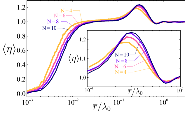
FIG. 3. \langle\eta\rangle is plotted as a function of \bar{r}/\lambda_0 for different values of N using a rate equation approximation for \bar{r}/\lambda_0 < 10^{-1} (averaged over 400 random configurations) and using a trajectory method simulation (averaged over 200 configurations) \bar{r}/\lambda_0 > 10^{-1} . (Inset) Enlargement of the region of CE.
